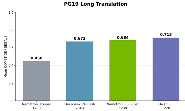
Figure 12 | Book level translation scores on the PG19 test set containing 100 books. Models are instructed to translate each book into German, Spanish, French, Italian, Japanese, and Chinese, forming 600 total translations. We then score each translation using the SEGAL (Wang et al., 2025a) pipeline.
