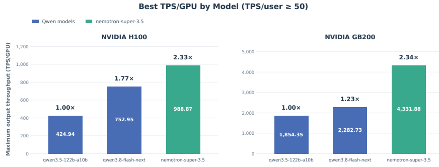
Figure 11 | Serving performance using vllm for the 20-turn agentic proxy workload, with 2K input tokens and 1K output tokens per turn. The graph shows the max-throughput of each model at \text{tps/user} \geq 50 .
