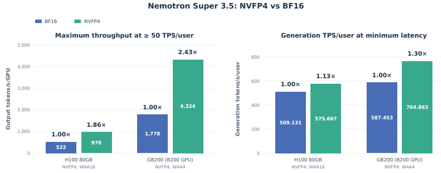
Figure 10 | Serving performance using vLLM on the 20-turn agentic proxy workload, with 2K input tokens and 1K output tokens per turn and ReplaySSM disabled. The graphs compare NVFP4 and BF16 maximum throughput at \geq 50 tokens/s/user and minimum latency.
