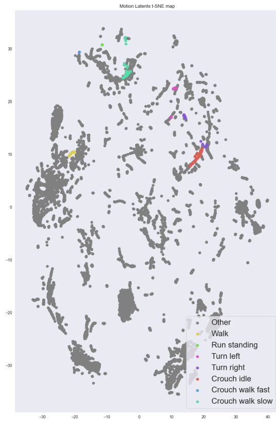
Fig. 10. CALM TSNE analysis
