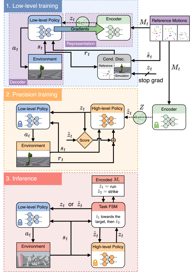
Fig. 2. The CALM framework consists of three phases. 1) In the initial training phase, both the encoder and low-level policy are developed by utilizing feedback from a conditional discriminator. The encoder learns to create a condensed representation that encapsulates the core of the motion, while the low-level policy, which interacts with the environment, serves as a decoder. 2) Once the pre-training phase has concluded, the encoder and low-level policy are frozen. The next step is precision training . Here, a high-level policy is trained to control the low-level policy. 3) In the last phase, inference , the high-level policy is also frozen. Solutions to complex tasks are then described using finite state machines (FSM), rule-based systems that do not require training, instead of rewards. Based on the state of the task, the FSM either provides a command to the high-level policy or provides a latent directly to the low-level policy.
