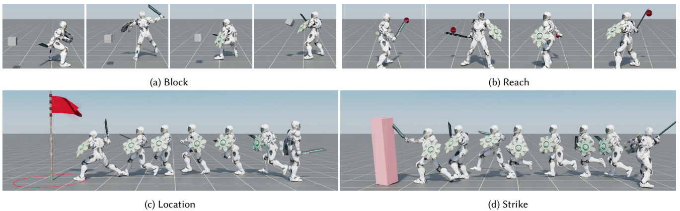
Fig. 8. Standard hierarchical task solving. A high-level policy directly controls the low-level policy and optimizes a task-specific objective.
