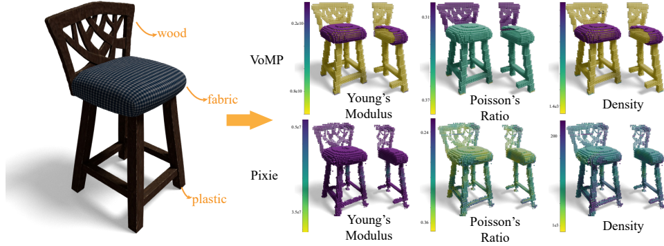
Figure 15: Comparing Estimations. We compare property estimates between VoMP and Pixie for a mesh.
