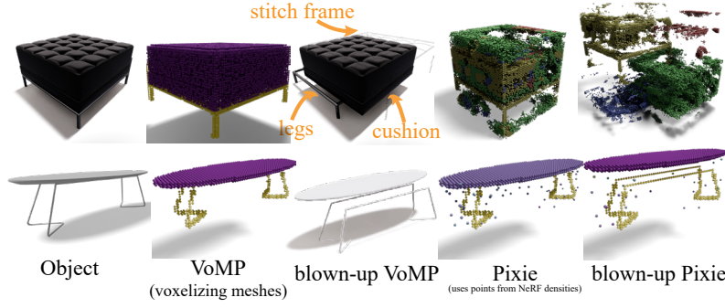
Figure 14: Data Annotation. We compare data annotation process of VoMP and Pixie.
