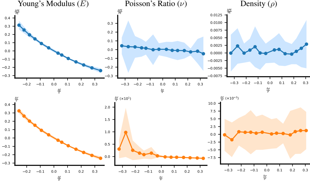
Figure 19: Tensile Testing Machine. We demonstrate the relation between relative errors in materials and relative change in P.E. (top) and volume (bottom). We show the confidence bounds in light shaded regions.
