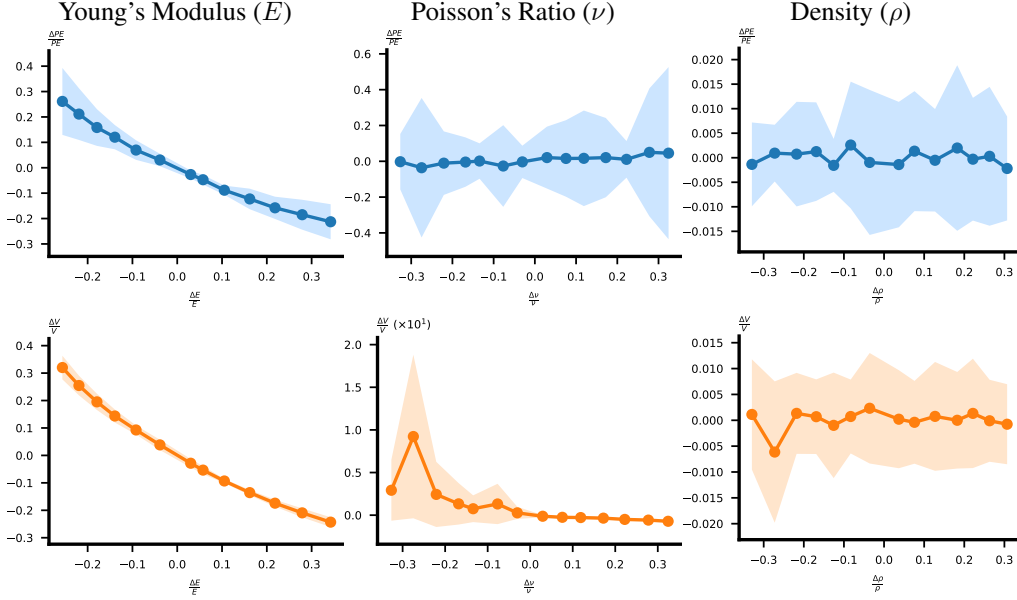
Figure 20: Tension. We demonstrate the relation between relative errors in materials and relative change in P.E. (top) and volume (bottom). We show the confidence bounds in light shaded regions.
