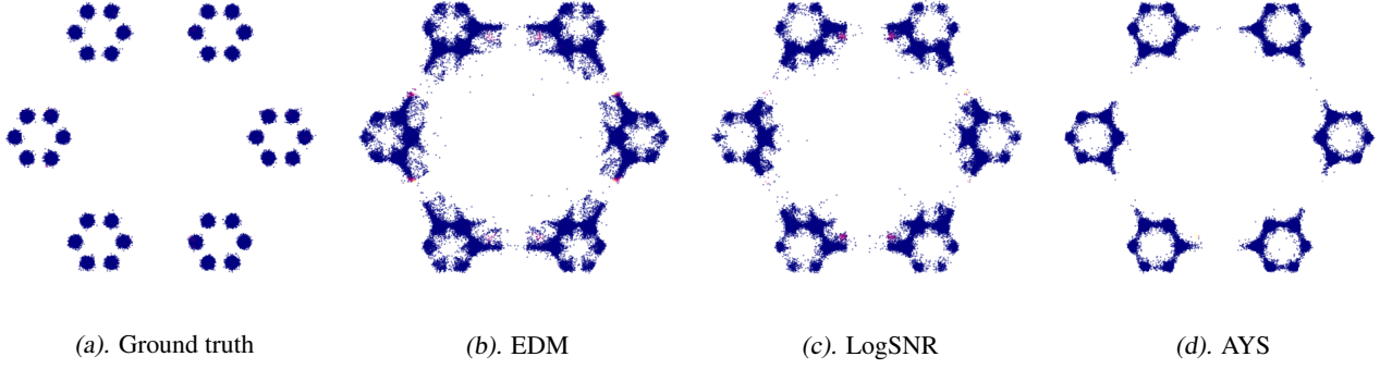
Figure 14. Modeling a 2D toy distribution: (a) Ground truth samples; (b), (c), and (d) are samples generated using 6 steps of Stochastic-DDIM with EDM, LogSNR, and AYS schedules, respectively. Each image consists of 100,000 sampled points.
