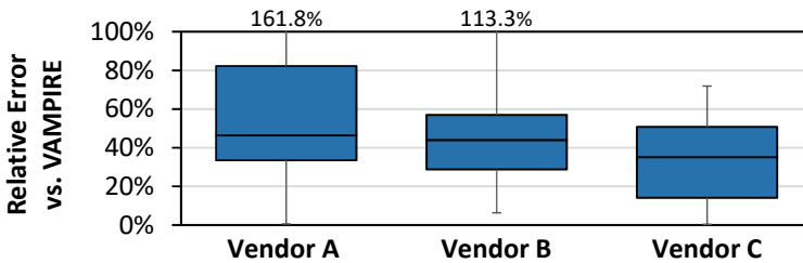
Fig. 25. Box plots showing the distribution of the relative error for the DRAMPower model compared to VAMPIRE, across the applications that we simulate. Each box illustrates the quartiles of the distribution of the relative error for each application, and the whiskers illustrate the minimum and maximum error values, across all applications evaluated.
