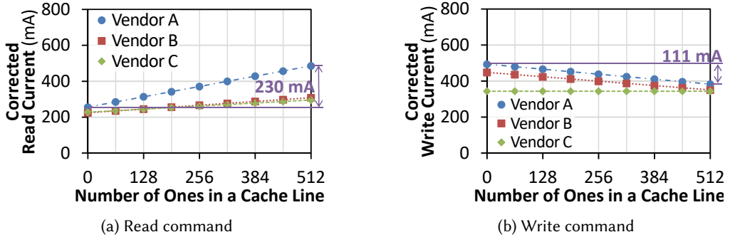
Fig. 16. Effect of the number of ones on the read (left) and write (right) current drawn by DRAM, after subtracting a conservative estimate of the I/O driver current.
