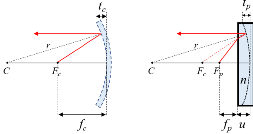
Fig. 9. (a) A spherical image combiner and (b) a planar image combiner with the same radius of curvature r . Note that the focal length of planar image combiner f_p is shorter than that of spherical image combiner f_c with the same thickness ( t_c = t_p )
