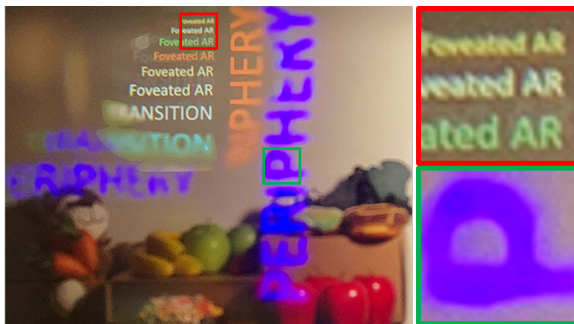
Fig. 17. Display photographed through the display of the wearable prototype. The top, red inset shows a detail from the foveal region and the lower, green inset is from the peripheral region. Note that the smaller projector used in the wearable prototype has narrower light cone angle and worse color representation which led to smaller FOV ( 77^\circ \times 53^\circ ) and severe color mismatch.
