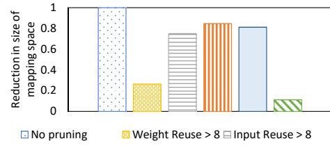
Fig. 7: Pruning heuristics and mapping space size.
