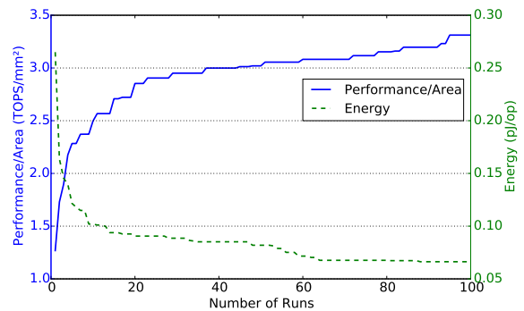
Fig. 8: Design quality achieved by iterating the MAGNet tuner. Results were averaged over 10 seeds.
